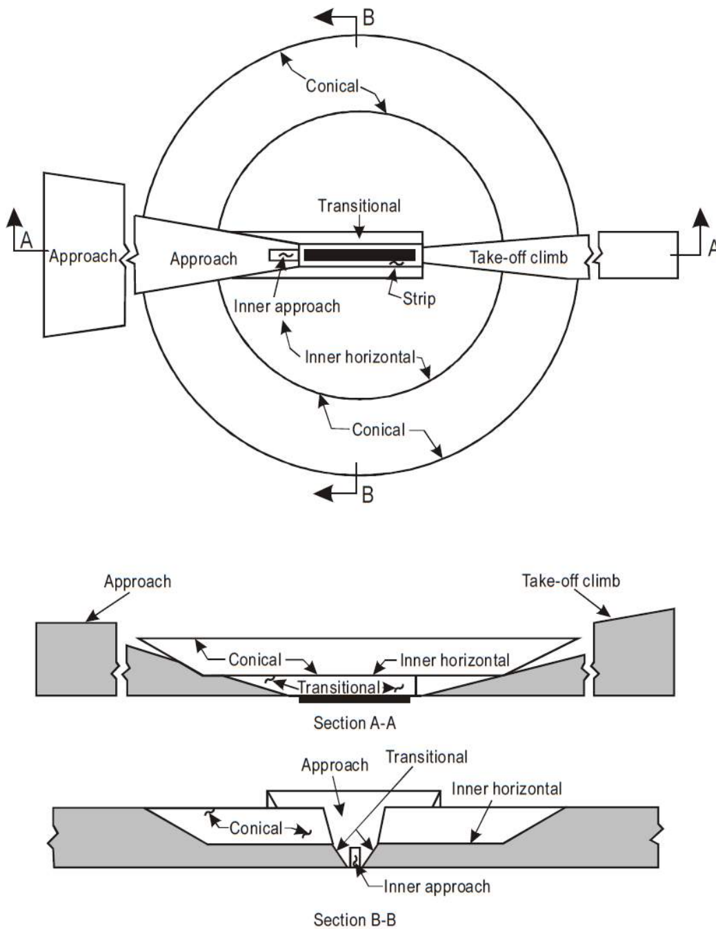
Figuur 2-1: ICAO obstakel beperkingsvlakken [2]
